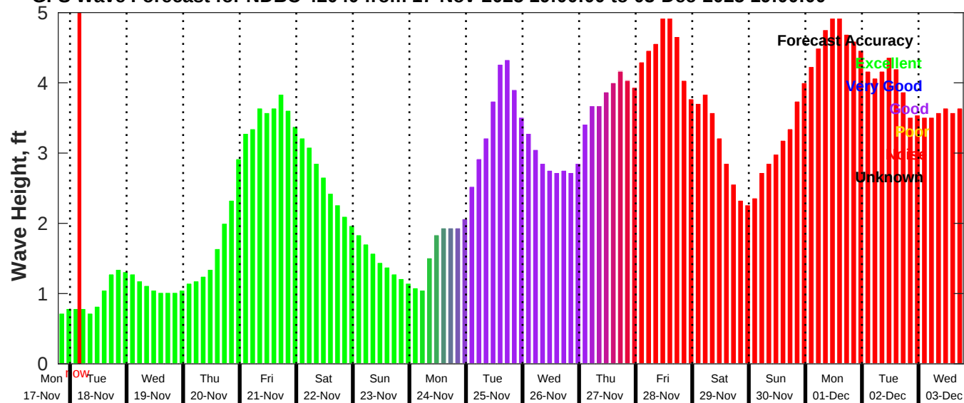
GFS Wave Forecast for NDBC 42040 from 17-Nov-2025 19:00:00 to 03-Dec-2025 19:00:00
