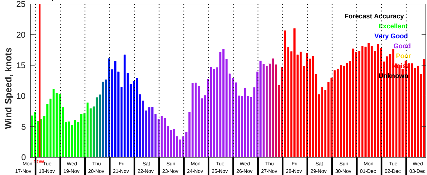
GFS Wind Speed Forecast for NDBC 42040 from 17-Nov-2025 19:00:00 to 03-Dec-2025 19:00:00
