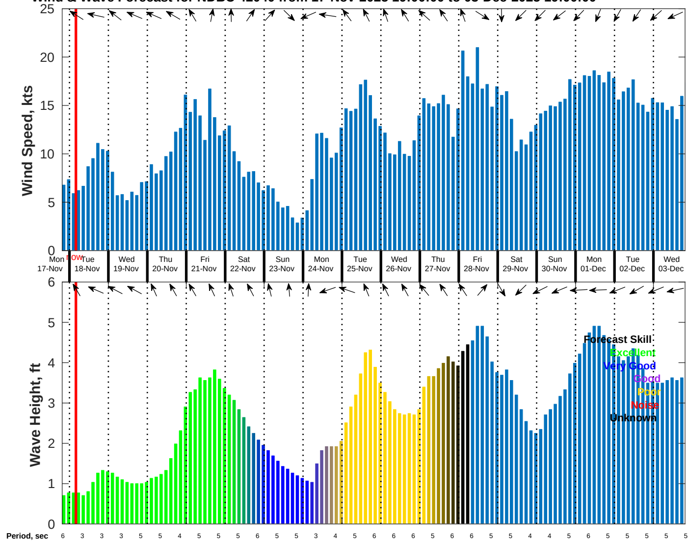
Wind & Wave Forecast for NDBC 42040 from 17-Nov-2025 19:00:00 to 03-Dec-2025 19:00:00
