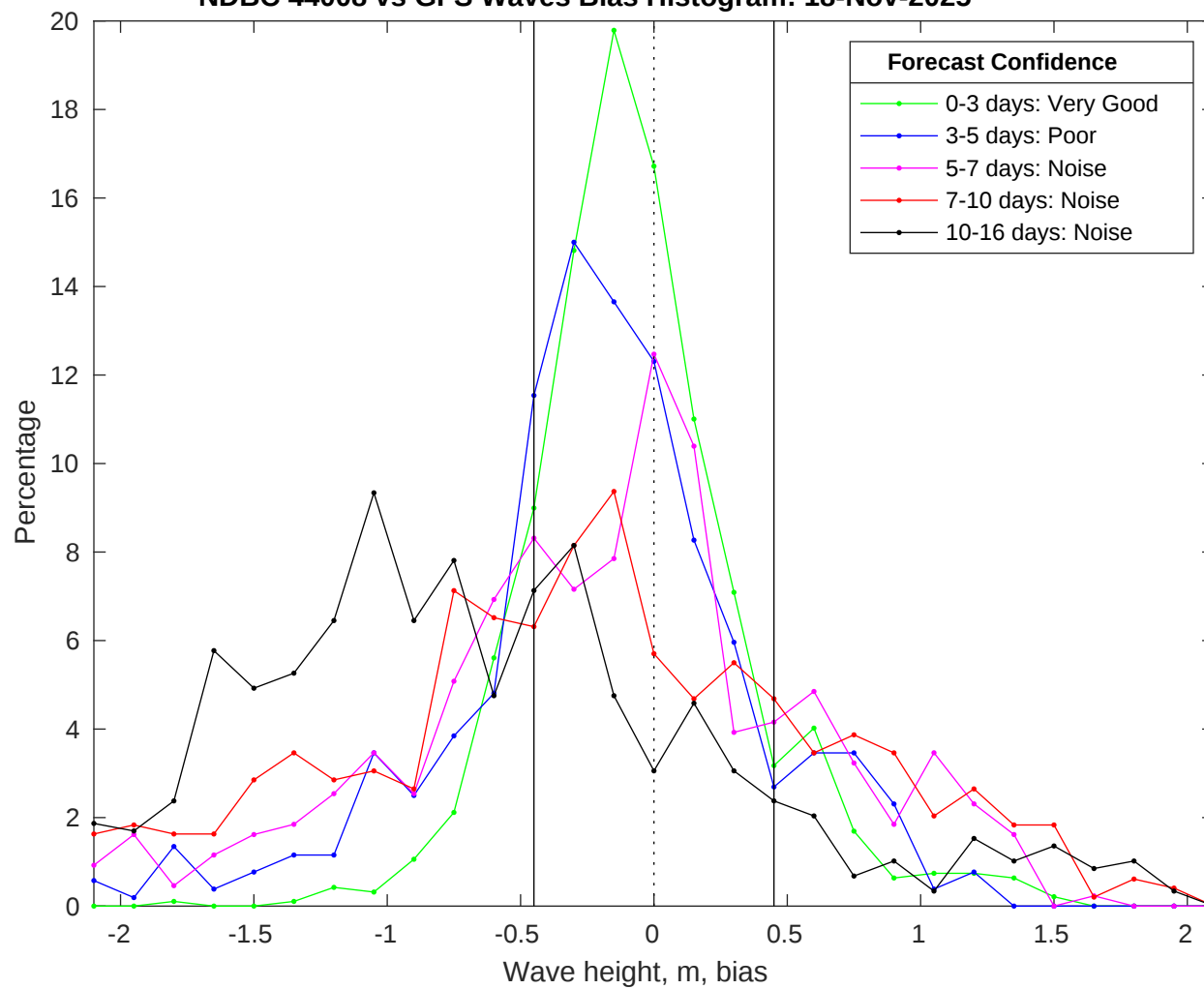
NDBC 44008 vs GFS Waves Bias Histogram: 18-Nov-2025
