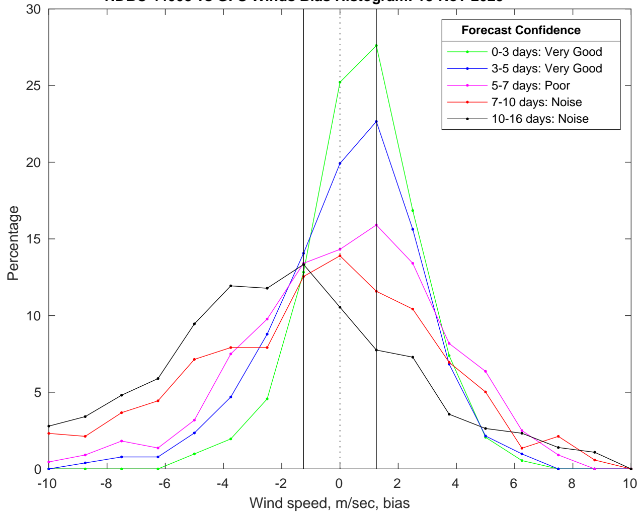
NDBC 44008 vs GFS Winds Bias Histogram: 18-Nov-2025
