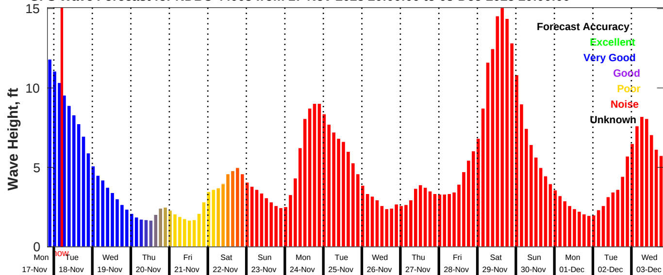
GFS Wave Forecast for NDBC 44008 from 17-Nov-2025 20:00:00 to 03-Dec-2025 20:00:00
