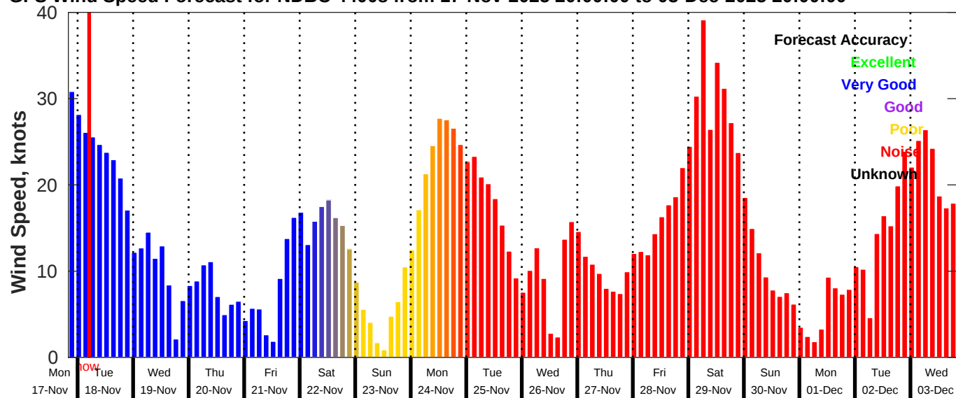
GFS Wind Speed Forecast for NDBC 44008 from 17-Nov-2025 20:00:00 to 03-Dec-2025 20:00:00
