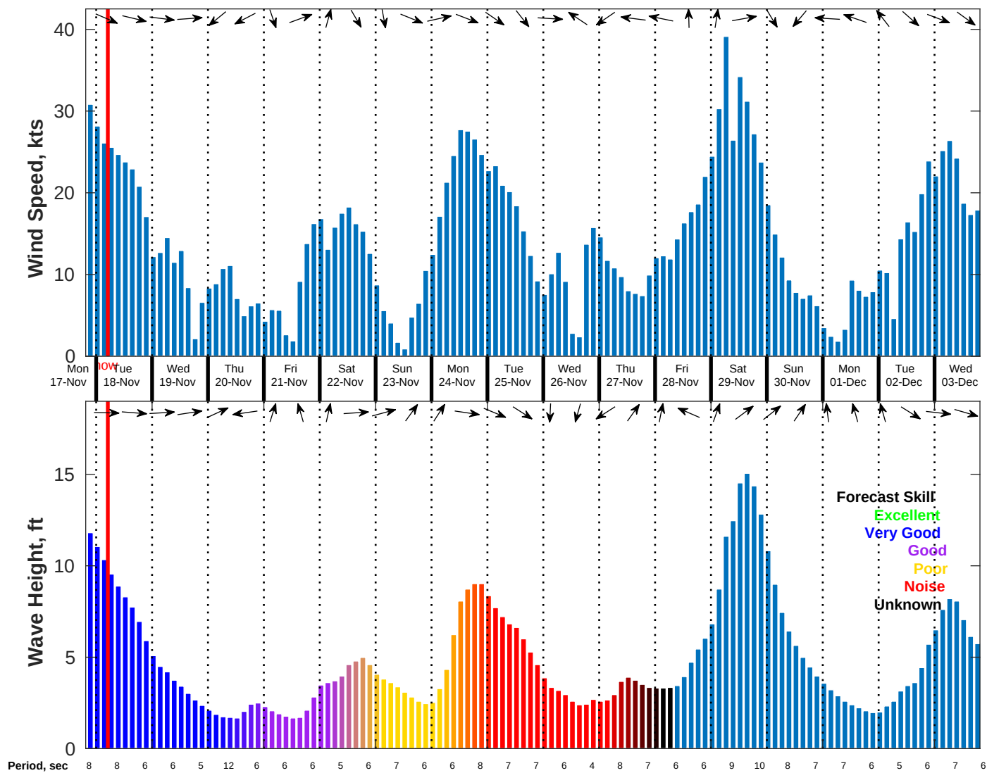
Wind & Wave Forecast for NDBC 44008 from 17-Nov-2025 20:00:00 to 03-Dec-2025 20:00:00
