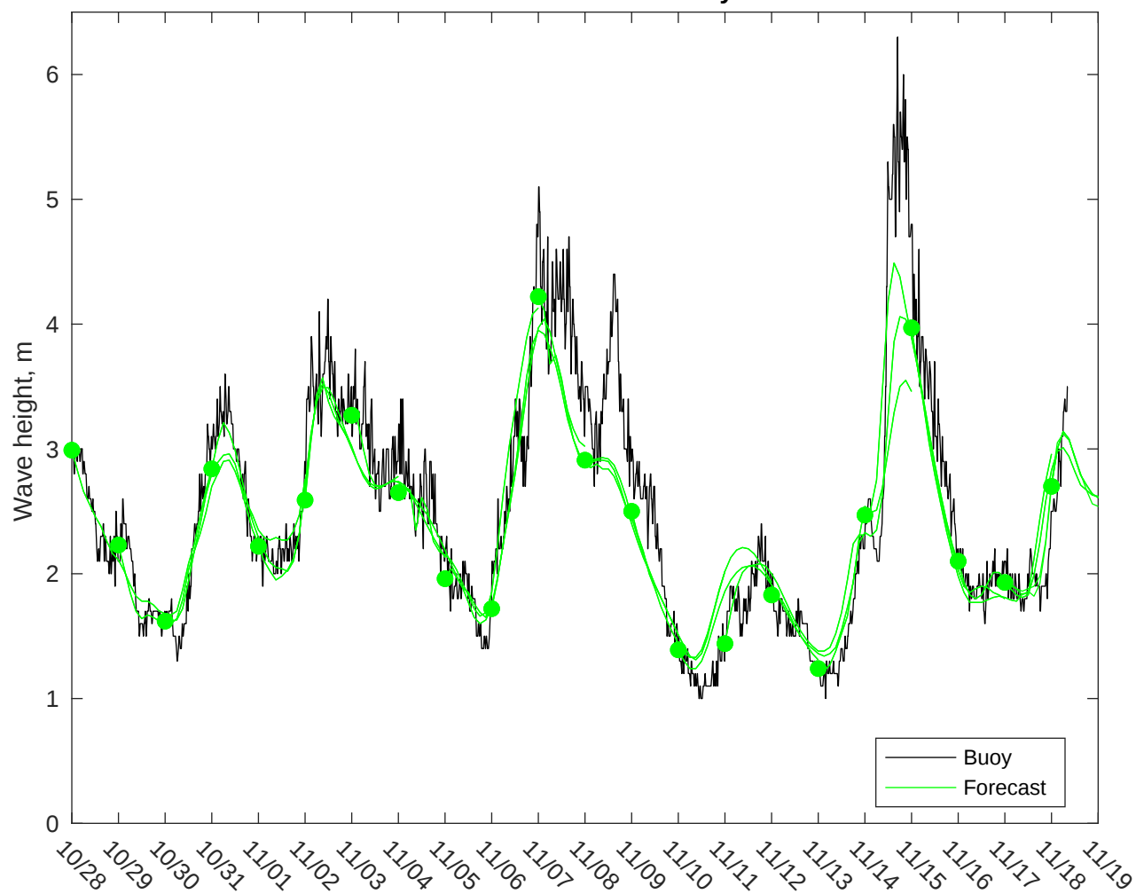
NDBC 46011 vs CMEMS Waves: 0 to 3 day forecast
