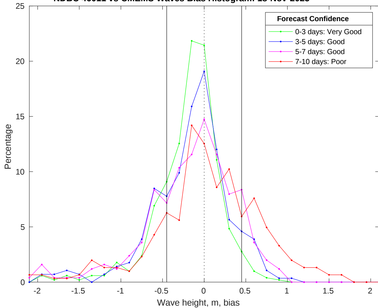
NDBC 46011 vs CMEMS Waves Bias Histogram: 18-Nov-2025
