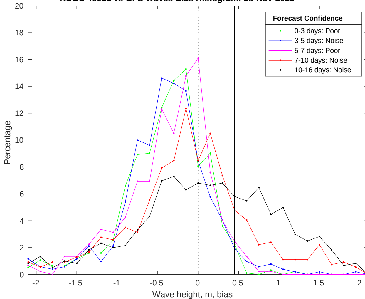
NDBC 46011 vs GFS Waves Bias Histogram: 18-Nov-2025
