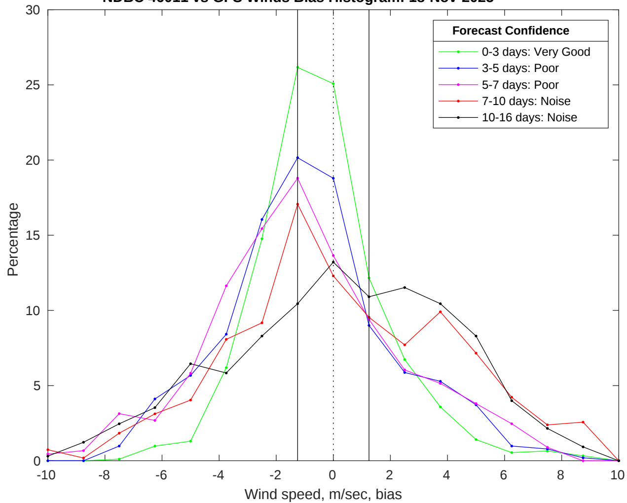
NDBC 46011 vs GFS Winds Bias Histogram: 18-Nov-2025
