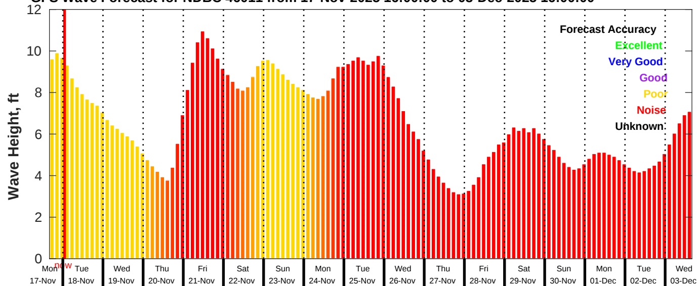
GFS Wave Forecast for NDBC 46011 from 17-Nov-2025 16:00:00 to 03-Dec-2025 16:00:00
