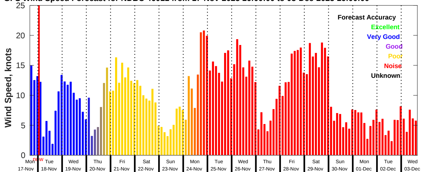
GFS Wind Speed Forecast for NDBC 46011 from 17-Nov-2025 16:00:00 to 03-Dec-2025 16:00:00
