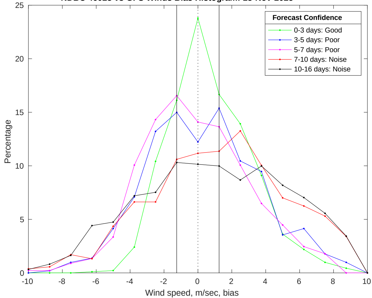
NDBC 46028 vs GFS Winds Bias Histogram: 18-Nov-2025
