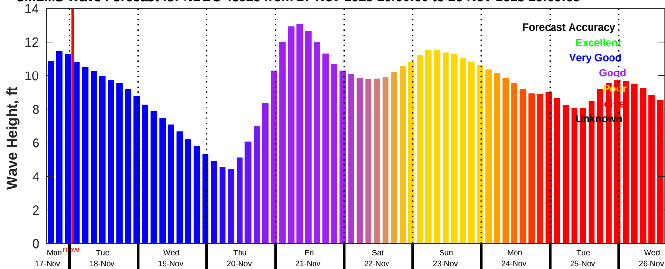
CMEMS Wave Forecast for NDBC 46028 from 17-Nov-2025 16:00:00 to 26-Nov-2025 16:00:00
