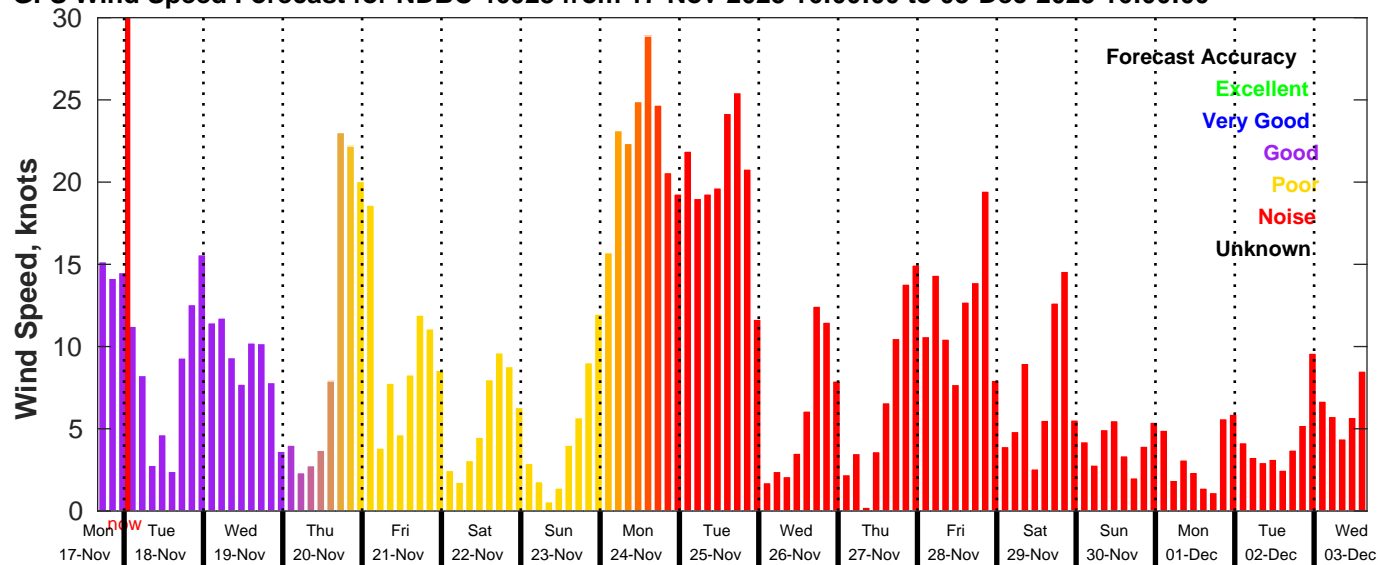
GFS Wind Speed Forecast for NDBC 46028 from 17-Nov-2025 16:00:00 to 03-Dec-2025 16:00:00
