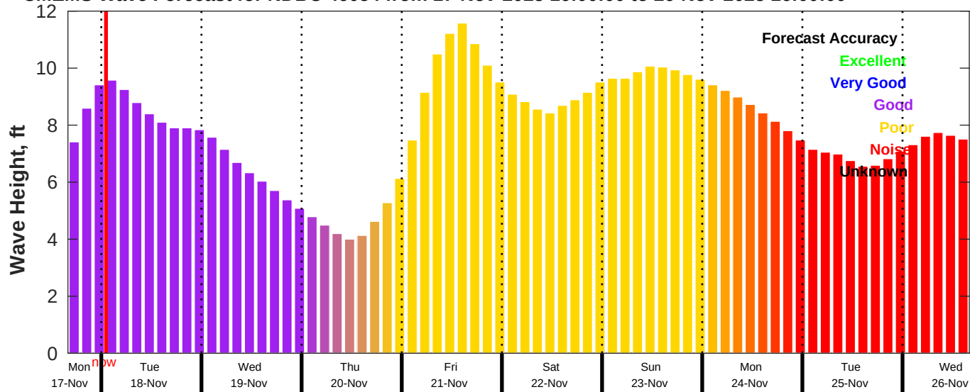
CMEMS Wave Forecast for NDBC 46054 from 17-Nov-2025 16:00:00 to 26-Nov-2025 16:00:00
