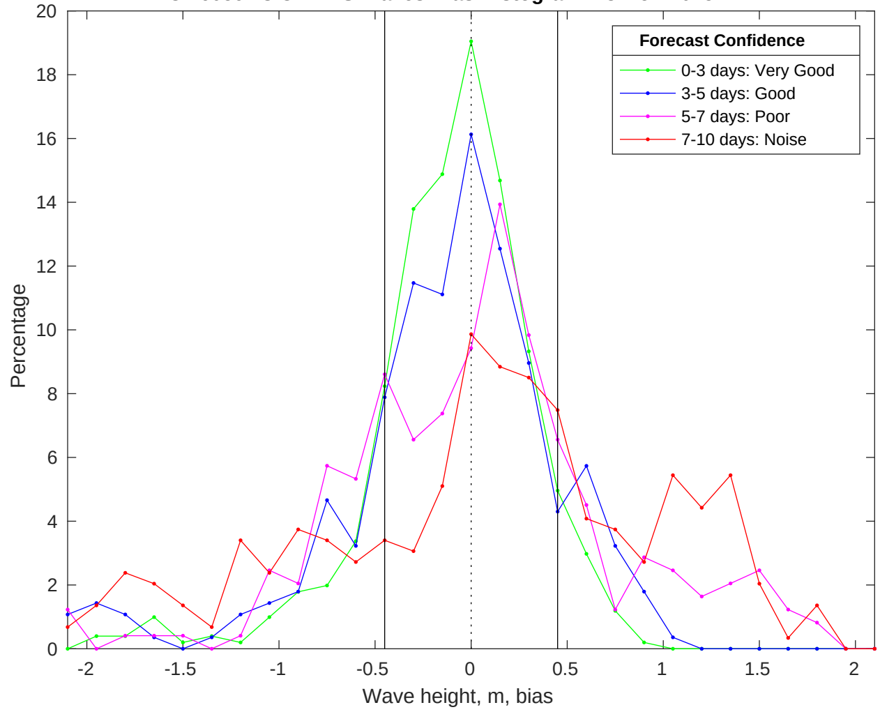
NDBC 46059 vs CMEMS Waves Bias Histogram: 18-Nov-2025
