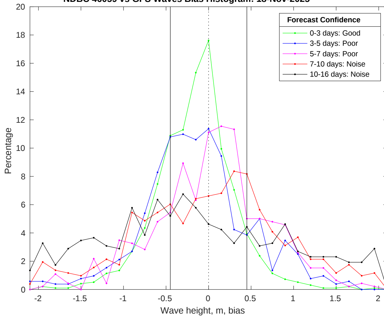
NDBC 46059 vs GFS Waves Bias Histogram: 18-Nov-2025
