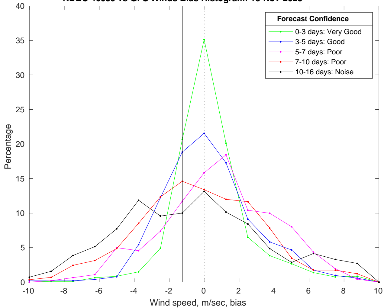
NDBC 46059 vs GFS Winds Bias Histogram: 18-Nov-2025
