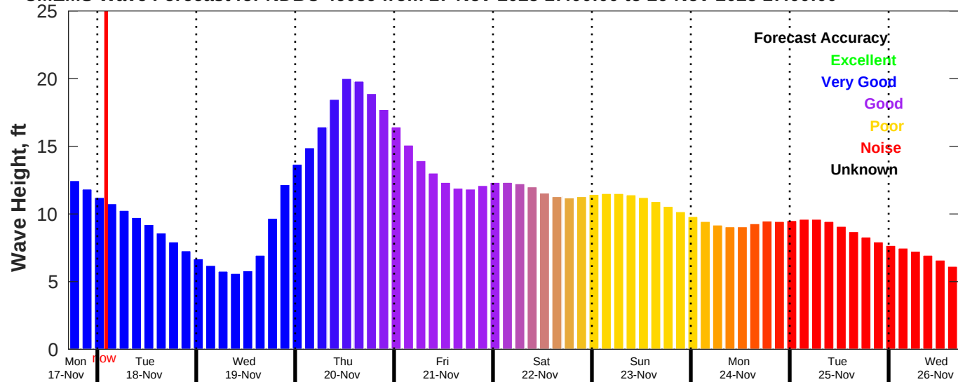
CMEMS Wave Forecast for NDBC 46059 from 17-Nov-2025 17:00:00 to 26-Nov-2025 17:00:00
