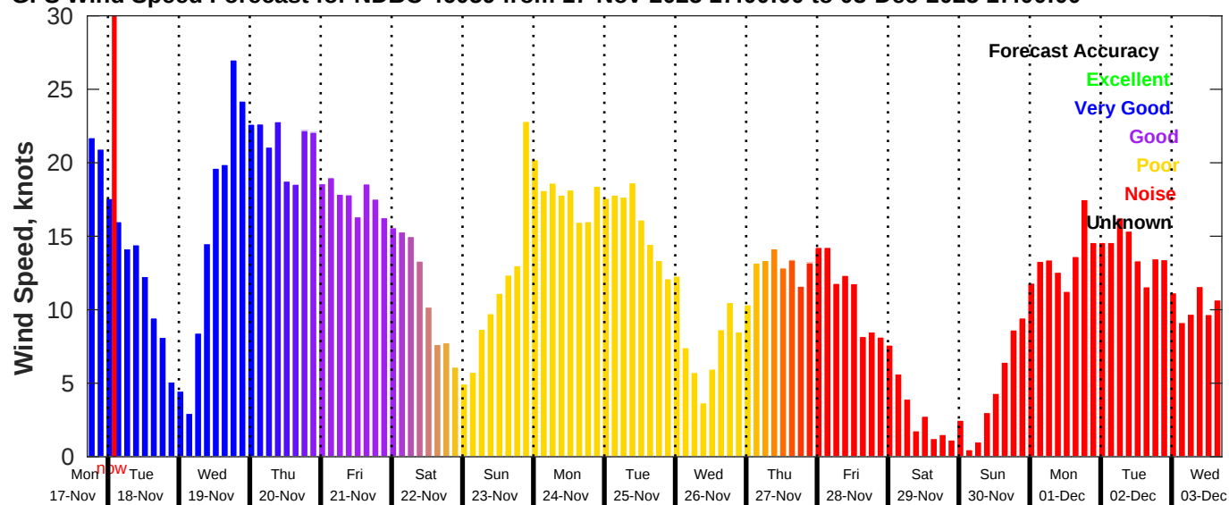
GFS Wind Speed Forecast for NDBC 46059 from 17-Nov-2025 17:00:00 to 03-Dec-2025 17:00:00
