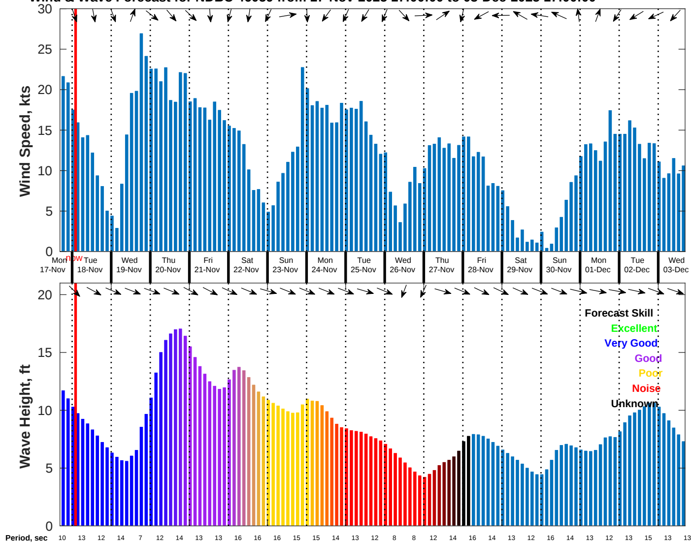
Wind & Wave Forecast for NDBC 46059 from 17-Nov-2025 17:00:00 to 03-Dec-2025 17:00:00
