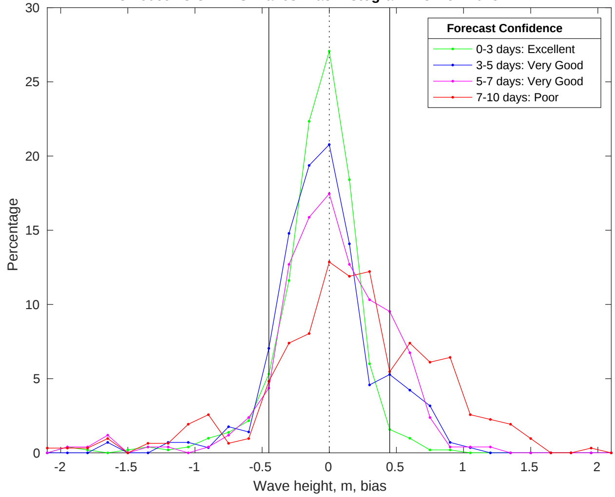
NDBC 46069 vs CMEMS Waves Bias Histogram: 18-Nov-2025
