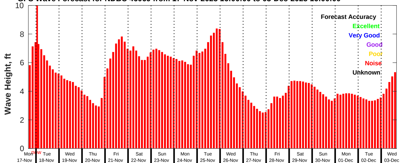
GFS Wave Forecast for NDBC 46069 from 17-Nov-2025 16:00:00 to 03-Dec-2025 16:00:00
