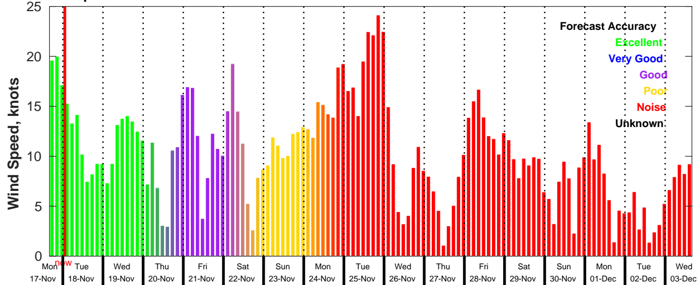
GFS Wind Speed Forecast for NDBC 46069 from 17-Nov-2025 16:00:00 to 03-Dec-2025 16:00:00
