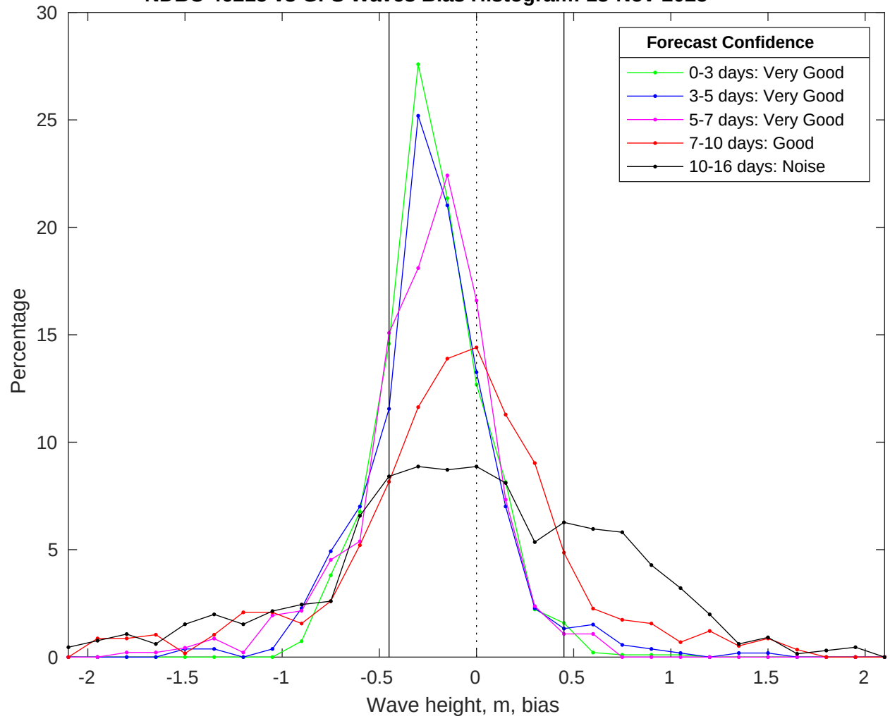
NDBC 46215 vs GFS Waves Bias Histogram: 18-Nov-2025
