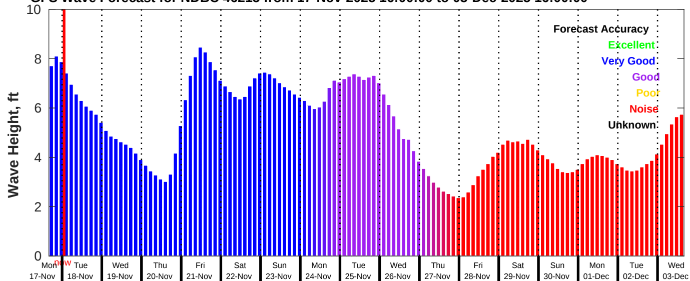
GFS Wave Forecast for NDBC 46215 from 17-Nov-2025 16:00:00 to 03-Dec-2025 16:00:00
