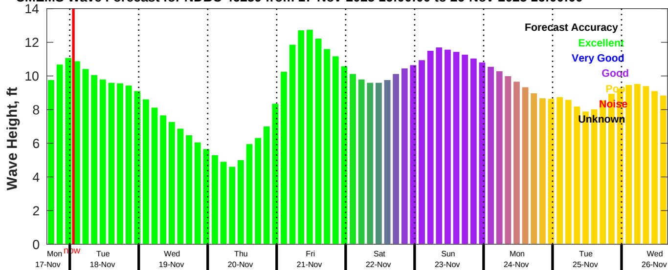
CMEMS Wave Forecast for NDBC 46259 from 17-Nov-2025 16:00:00 to 26-Nov-2025 16:00:00
