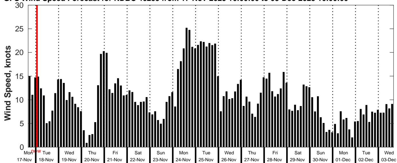
GFS Wind Speed Forecast for NDBC 46259 from 17-Nov-2025 16:00:00 to 03-Dec-2025 16:00:00
