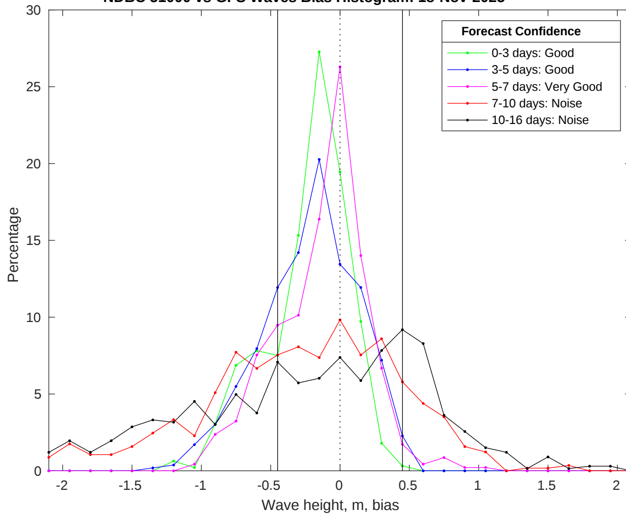
NDBC 51000 vs GFS Waves Bias Histogram: 18-Nov-2025
