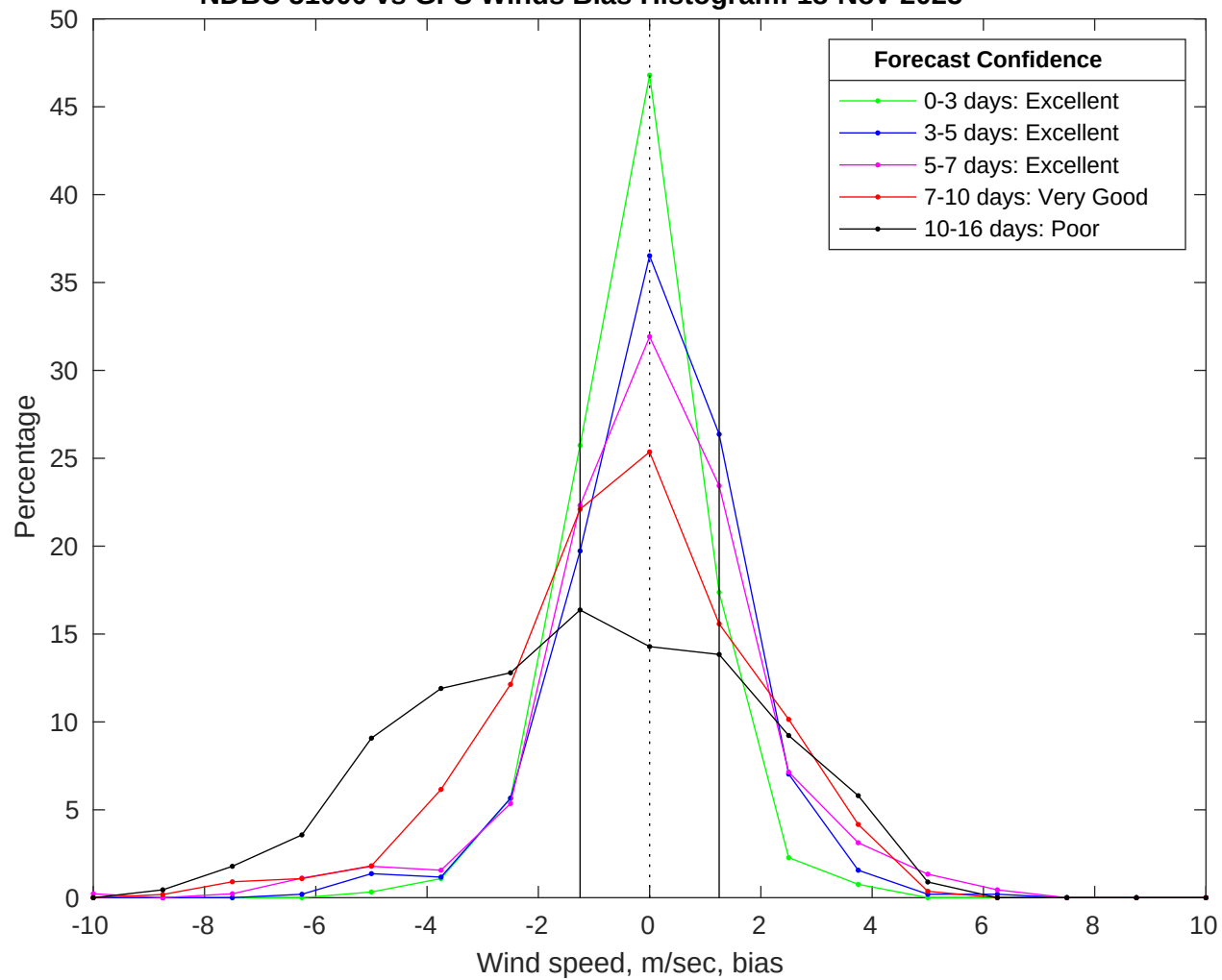
NDBC 51000 vs GFS Winds Bias Histogram: 18-Nov-2025
