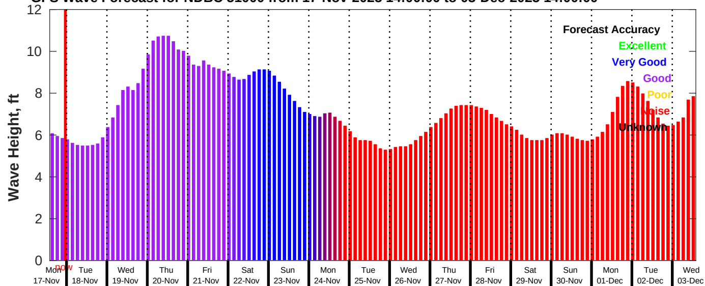
GFS Wave Forecast for NDBC 51000 from 17-Nov-2025 14:00:00 to 03-Dec-2025 14:00:00
