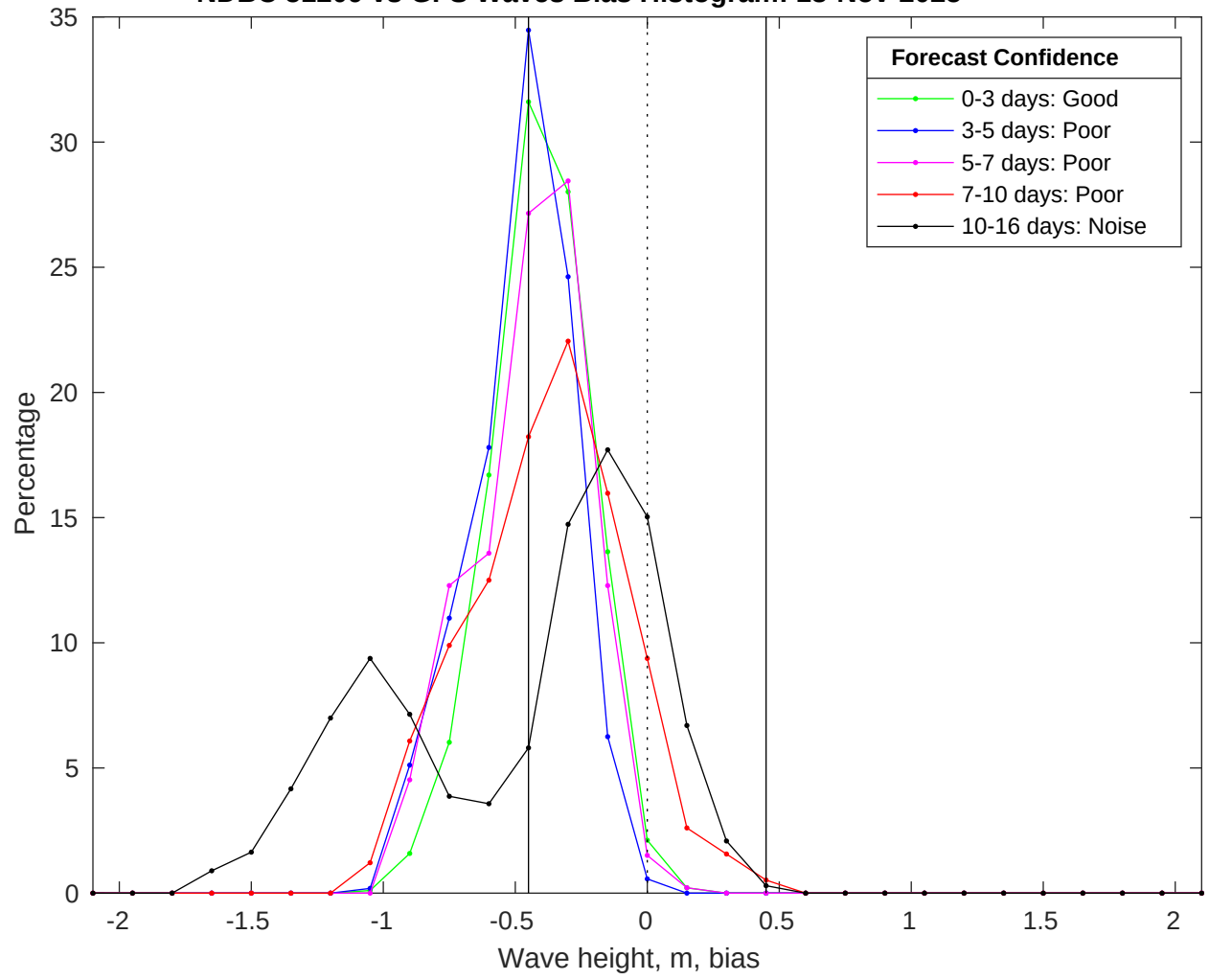
NDBC 51209 vs GFS Waves Bias Histogram: 18-Nov-2025
