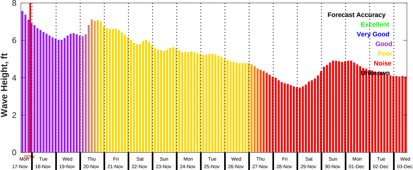
GFS Wave Forecast for NDBC 51209 from 17-Nov-2025 13:00:00 to 03-Dec-2025 13:00:00
