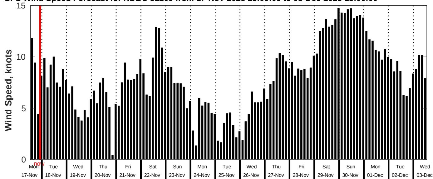
GFS Wind Speed Forecast for NDBC 51209 from 17-Nov-2025 13:00:00 to 03-Dec-2025 13:00:00
