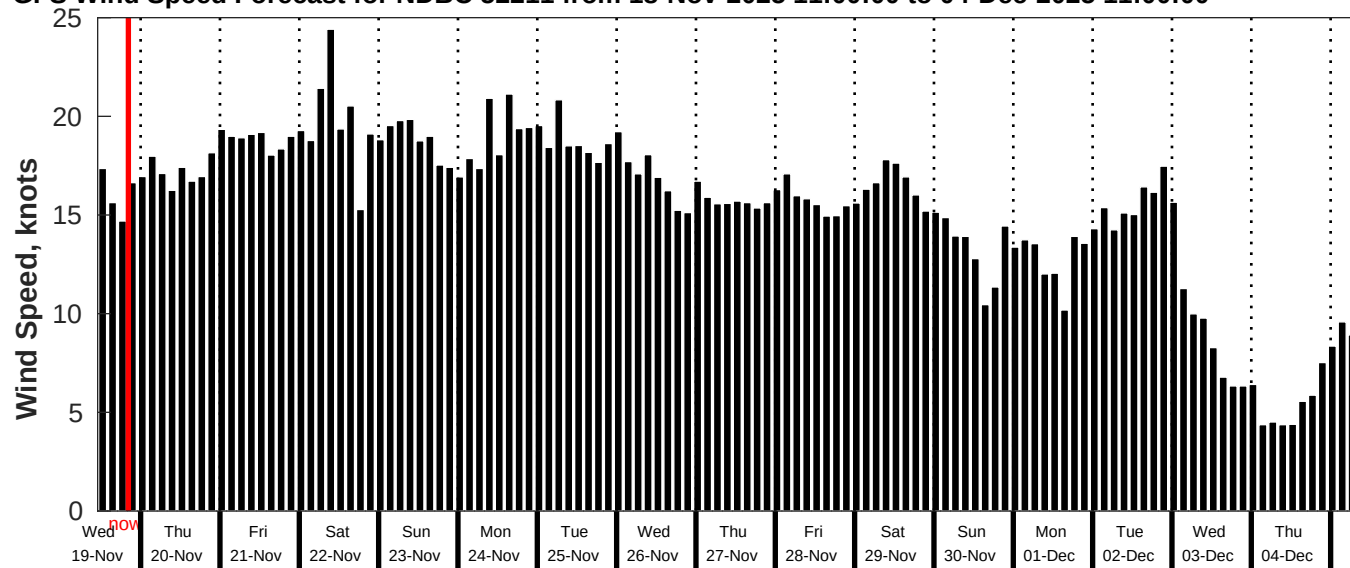
GFS Wind Speed Forecast for NDBC 52211 from 18-Nov-2025 11:00:00 to 04-Dec-2025 11:00:00
