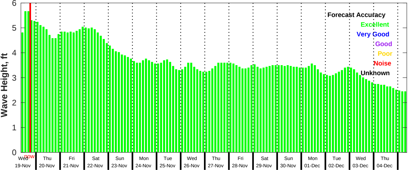
GFS Wave Forecast for NDBC 52212 from 18-Nov-2025 09:00:00 to 04-Dec-2025 09:00:00
