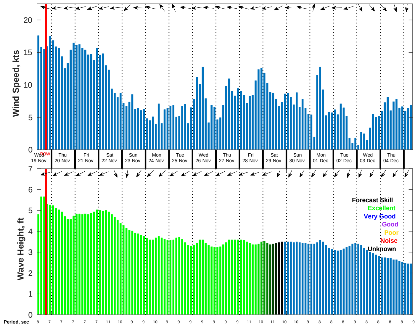
Wind & Wave Forecast for NDBC 52212 from 18-Nov-2025 09:00:00 to 04-Dec-2025 09:00:00
