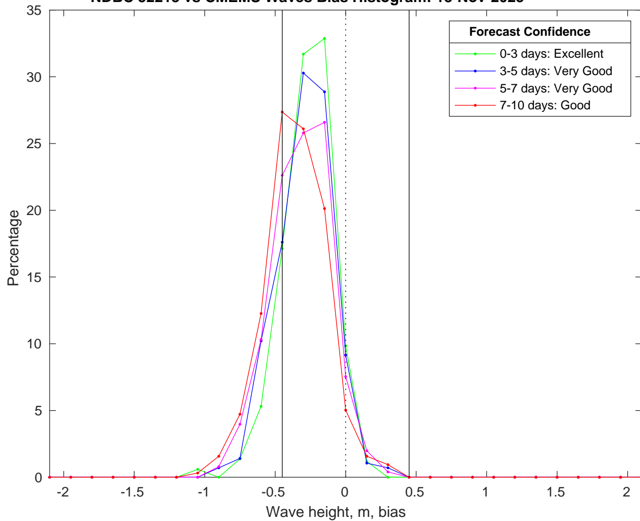
NDBC 52213 vs CMEMS Waves Bias Histogram: 18-Nov-2025
