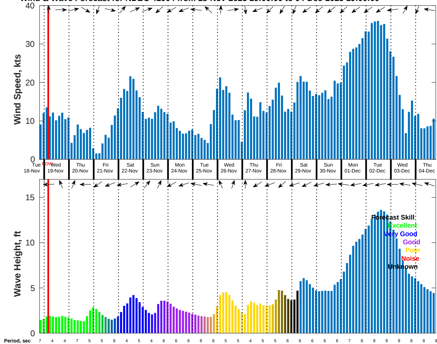
Wind & Wave Forecast for NDBC 41004 from 18-Nov-2025 19:00:00 to 04-Dec-2025 19:00:00
