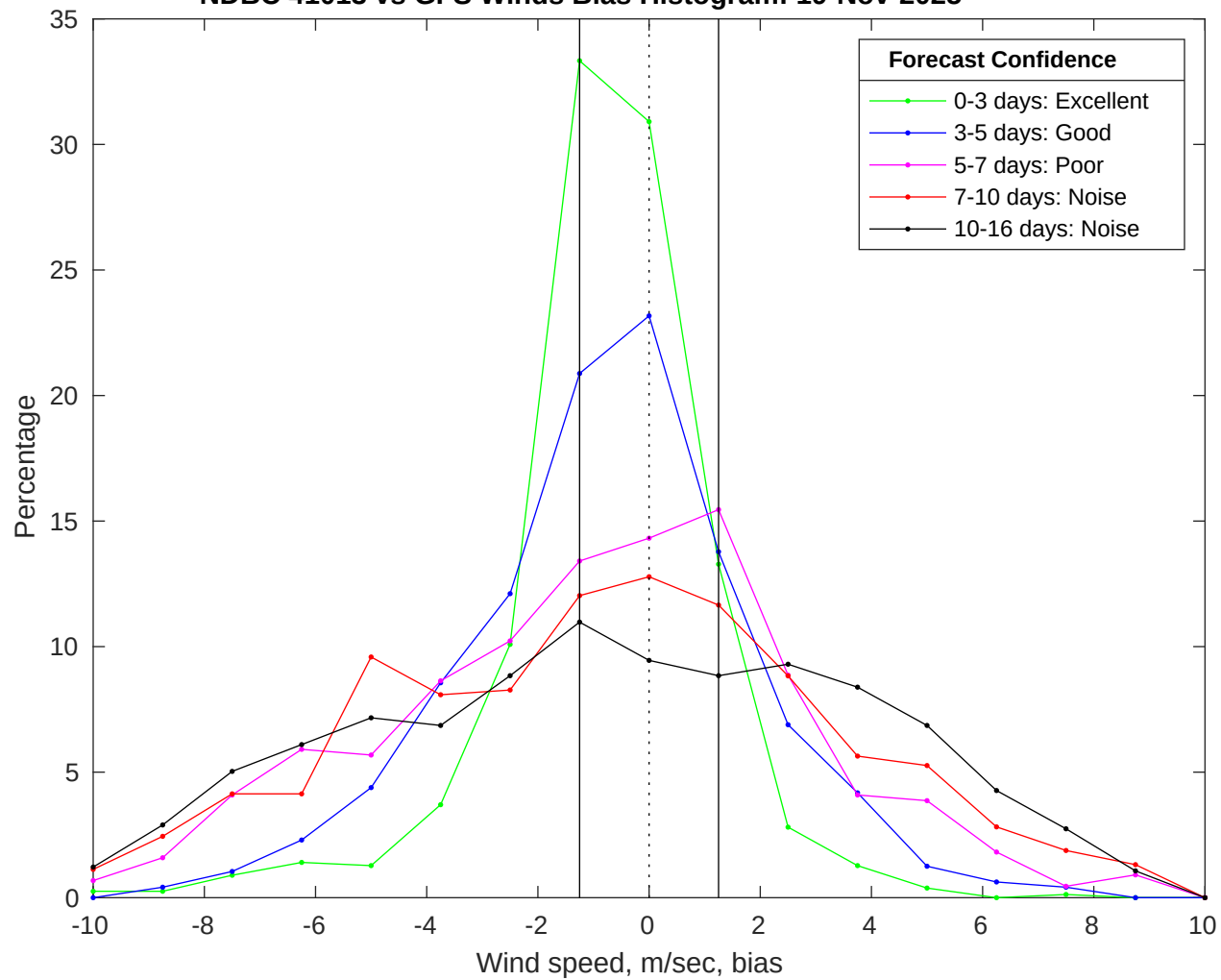
NDBC 41013 vs GFS Winds Bias Histogram: 19-Nov-2025
