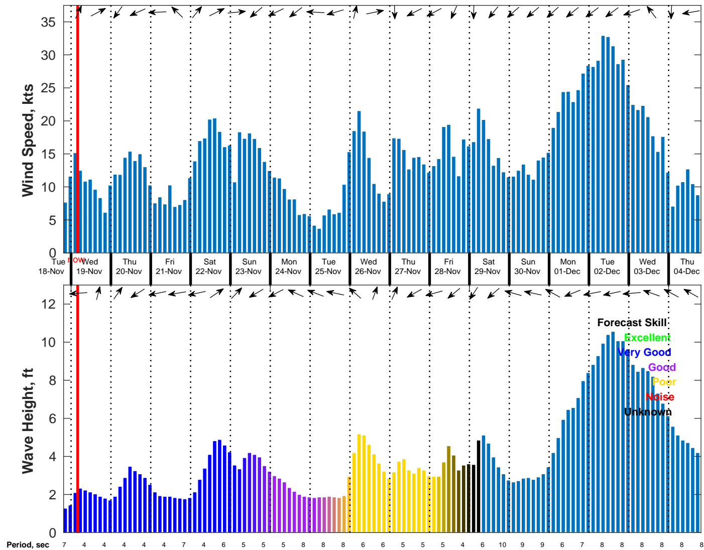
Wind & Wave Forecast for NDBC 41013 from 18-Nov-2025 19:00:00 to 04-Dec-2025 19:00:00
