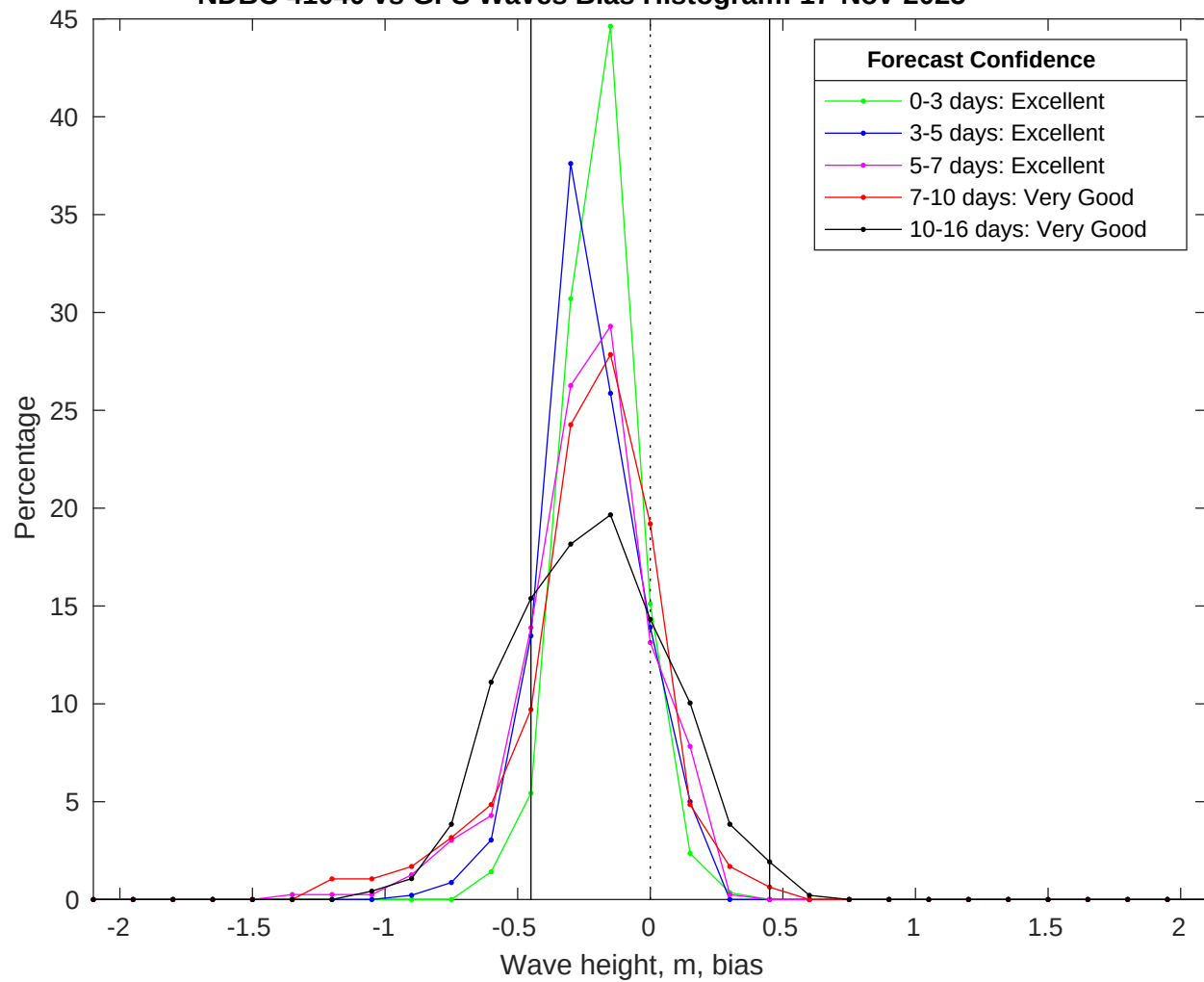
NDBC 41040 vs GFS Waves Bias Histogram: 17-Nov-2025
