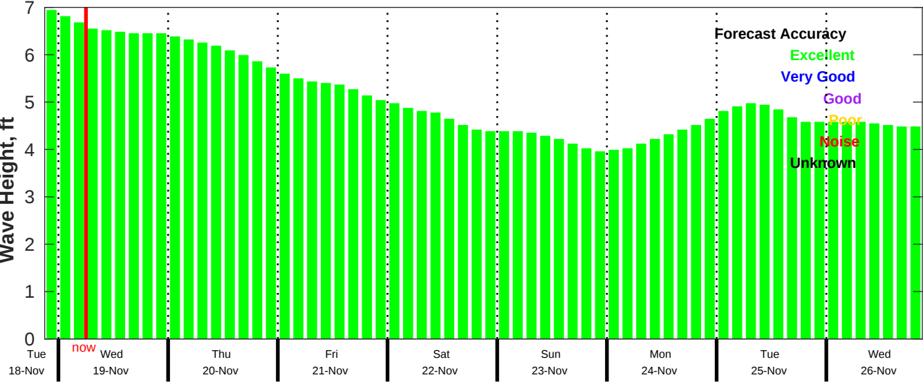
CMEMS Wave Forecast for NDBC 41040 from 18-Nov-2025 21:00:00 to 26-Nov-2025 21:00:00
