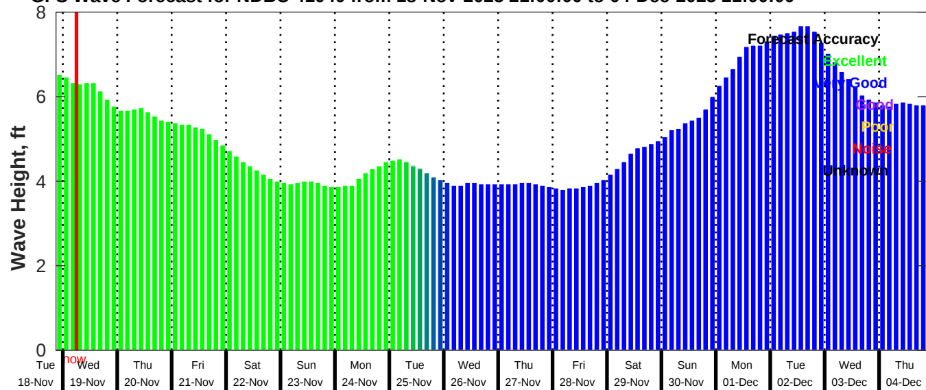
GFS Wave Forecast for NDBC 41040 from 18-Nov-2025 21:00:00 to 04-Dec-2025 21:00:00
