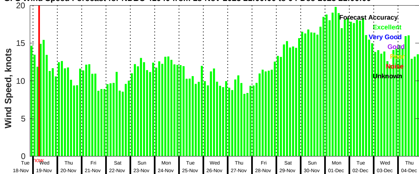
GFS Wind Speed Forecast for NDBC 41040 from 18-Nov-2025 21:00:00 to 04-Dec-2025 21:00:00
