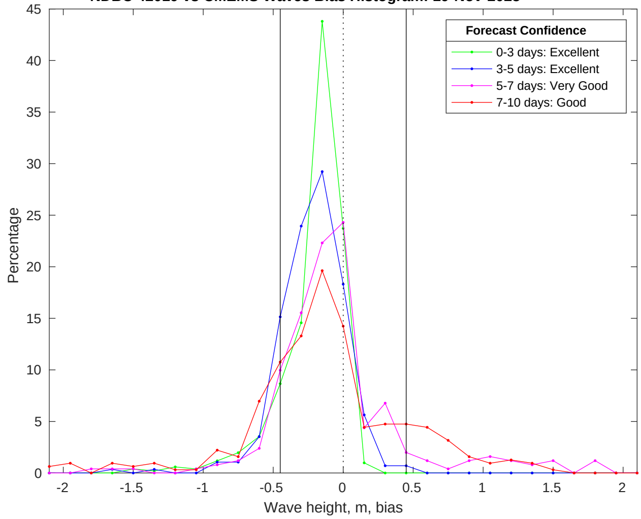
NDBC 42019 vs CMEMS Waves Bias Histogram: 19-Nov-2025
