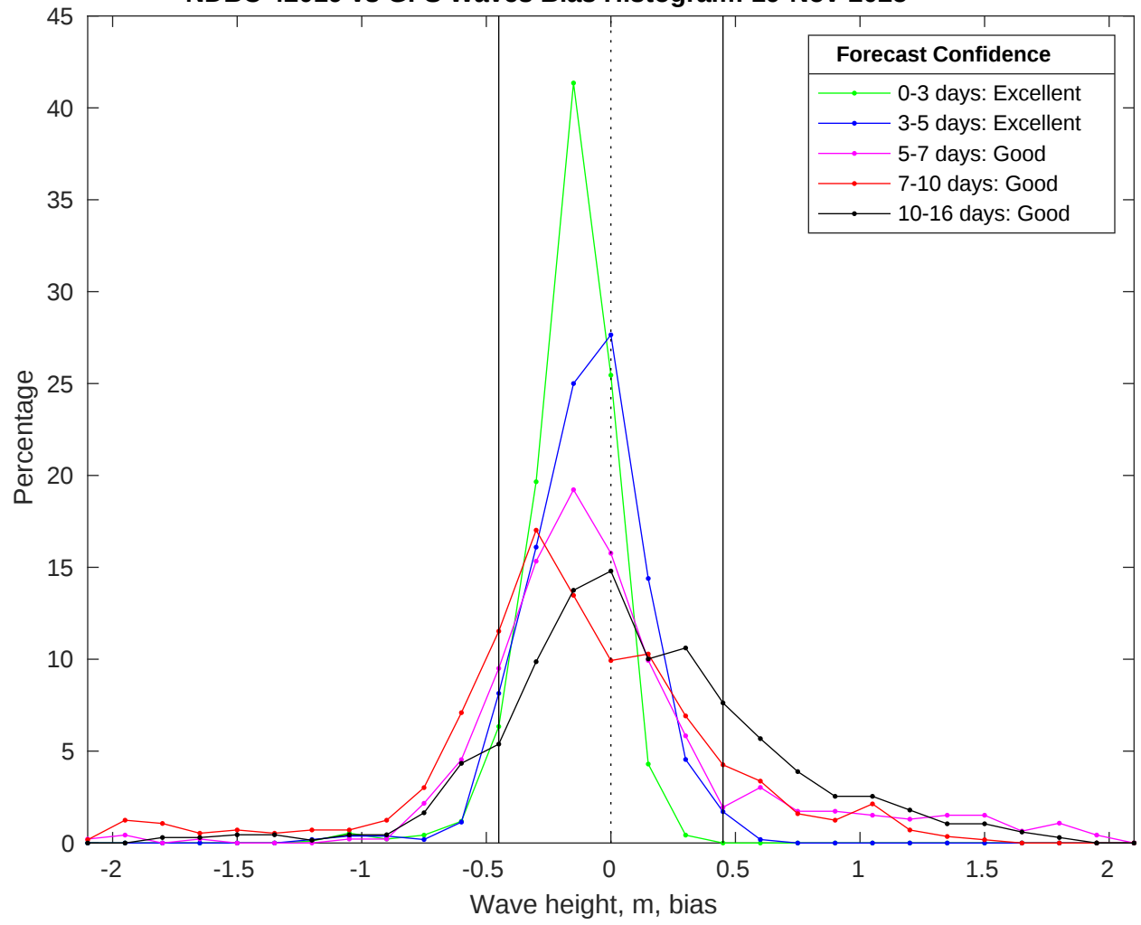
NDBC 42019 vs GFS Waves Bias Histogram: 19-Nov-2025
